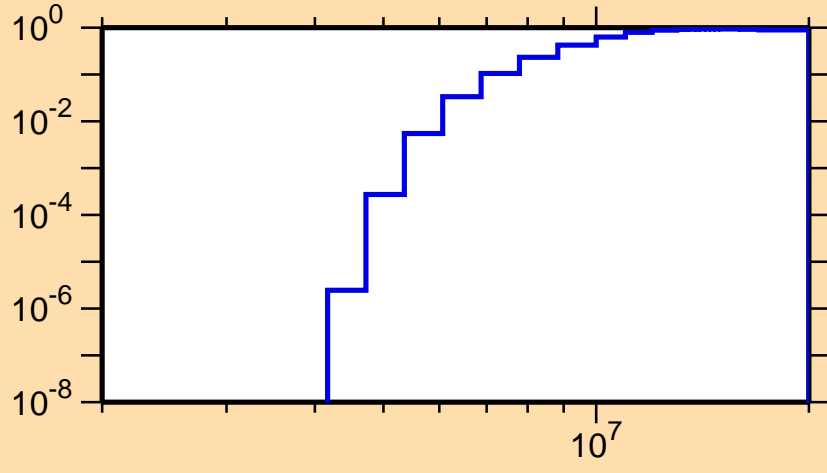
\sigma vs. E for ^{104}\text{In}(n,np)
