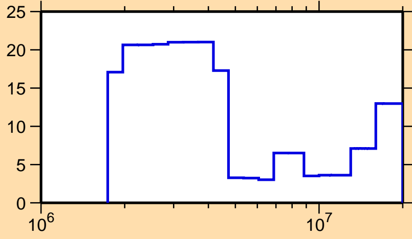
\Delta\sigma/\sigma vs. E for ^{104}\text{In}(n, el.)
