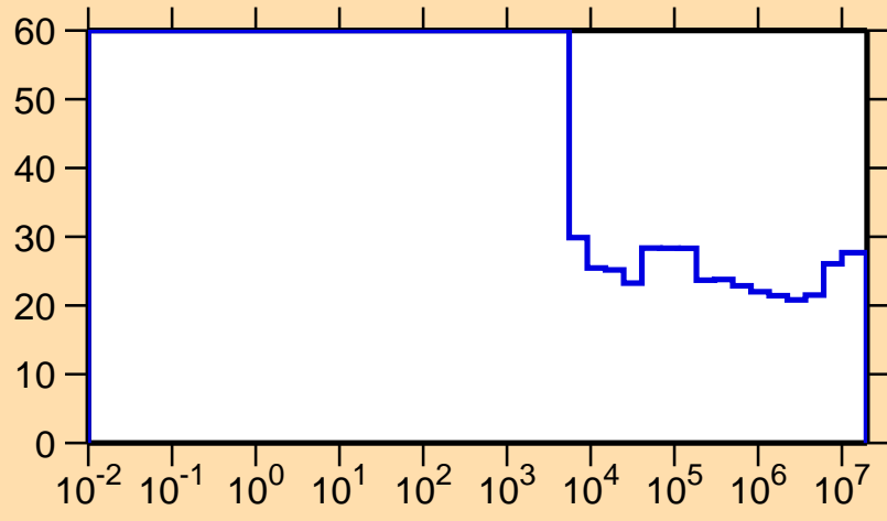
\Delta\sigma/\sigma vs. E for ^{104}\text{In}(n,p)
