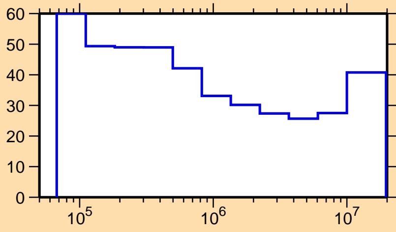
\Delta\sigma/\sigma vs. E for ^{104}\text{In}(n,n_1)
