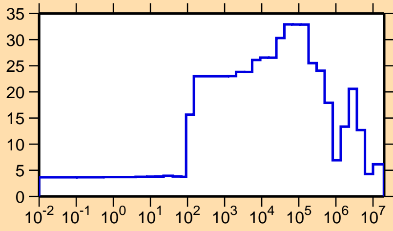
\Delta\sigma/\sigma vs. E for ^{104}\text{In}(n,el.)
