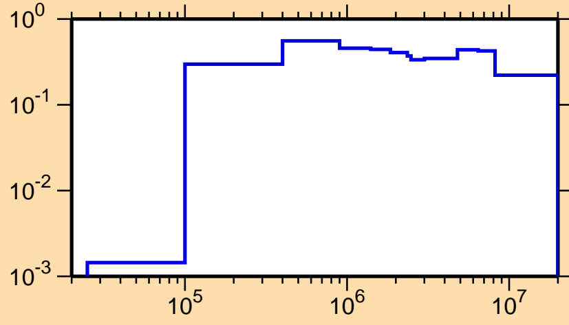
\sigma vs. E for ^{104}\text{In}(n,\text{inel.})
