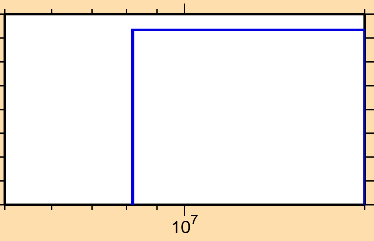
\sigma vs. E for ^{104}\text{In}(n,2np)
