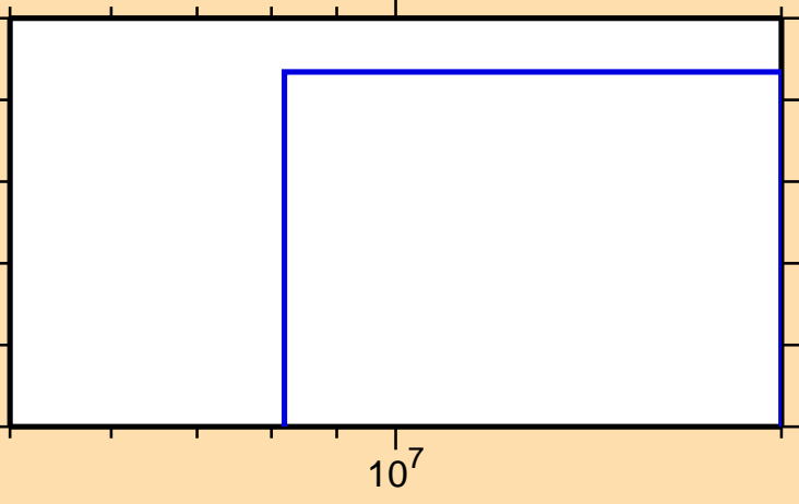
\sigma vs. E for ^{105}\text{In}(n,2np)
