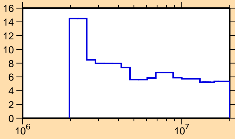
\Delta\sigma/\sigma vs. E for ^{105}\text{In}(n, n_{\text{nonel}})
