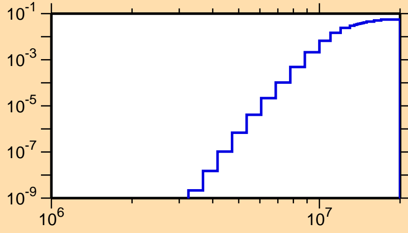
\sigma vs. E for ^{105}\text{In}(n,p\alpha)
