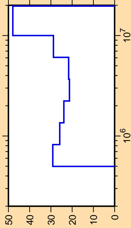
\Delta\sigma/\sigma vs. E for ^{105}\text{In}(n,n_4)
