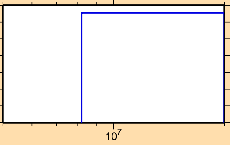
\sigma vs. E for ^{105}\text{In}(n,2n\alpha)
