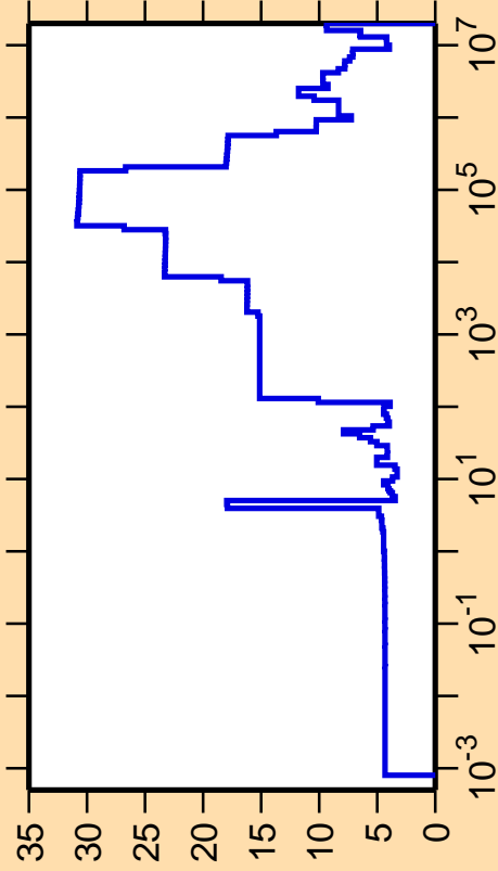
\Delta\sigma/\sigma vs. E for ^{106}\text{In}(n,\text{el.})
