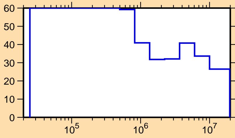
\Delta\sigma/\sigma vs. E for ^{106}\text{In}(n,n_1)
