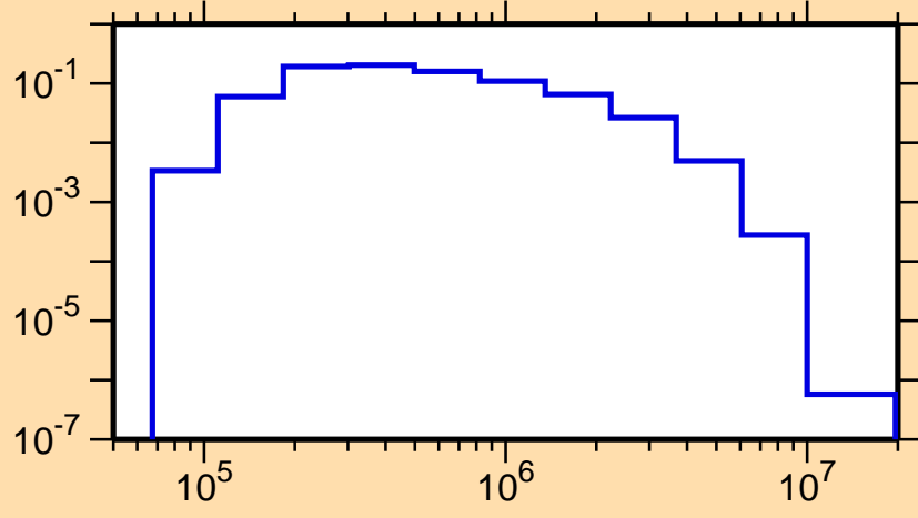
\sigma vs. E for ^{106}\text{In}(n,n_2)
