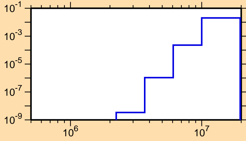
\sigma vs. E for ^{106}\text{In}(n,p)\alpha
