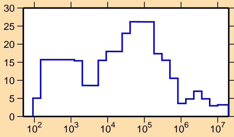
\Delta\sigma/\sigma vs. E for ^{106}\text{In}(n,\text{tot.})
