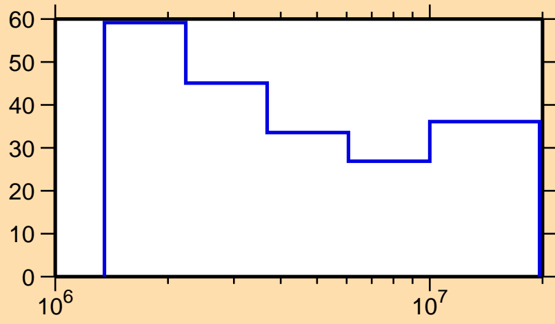
\Delta\sigma/\sigma vs. E for ^{106}\text{In}(n,n\text{cont.})
