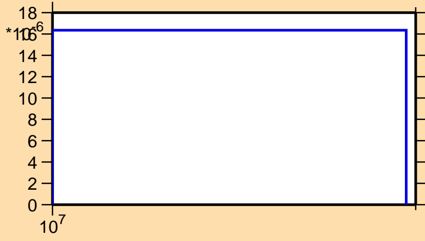
\sigma vs. E for ^{106}\text{In}(n,nd)
