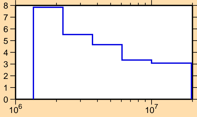
\Delta\sigma/\sigma vs. E for ^{106}\text{In}(n, n_{\text{nonel}})
