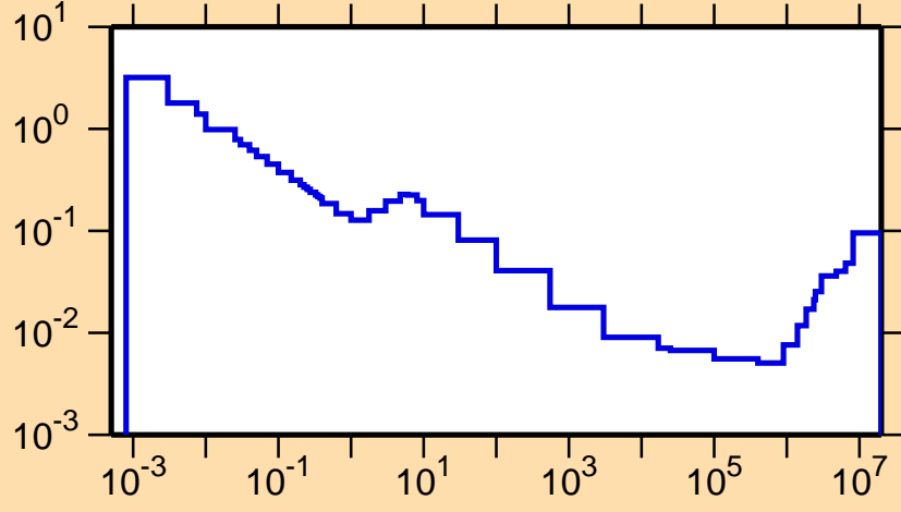
\sigma vs. E for ^{106}\text{In}(n,\alpha)
