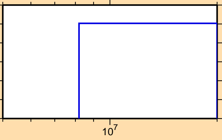
\sigma vs. E for ^{106}\text{In}(\text{mt117})
