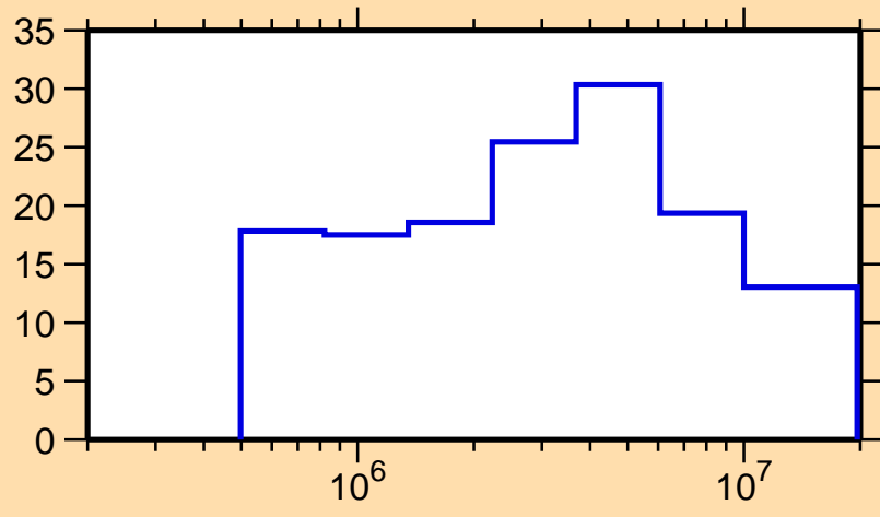
\Delta\sigma/\sigma vs. E for ^{107}\text{In}(n,n_1)
