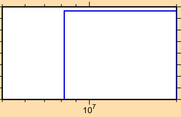
\sigma vs. E for ^{107}\text{In}(n,2np)
