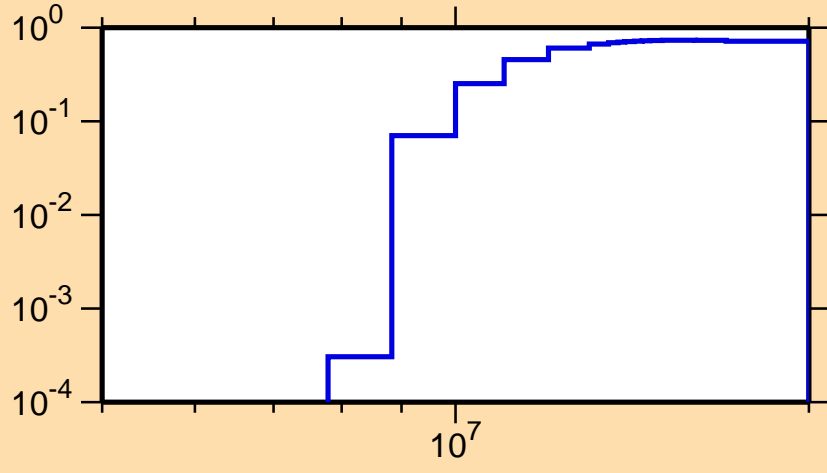
\sigma vs. E for ^{108}\text{In}(n,2n)
