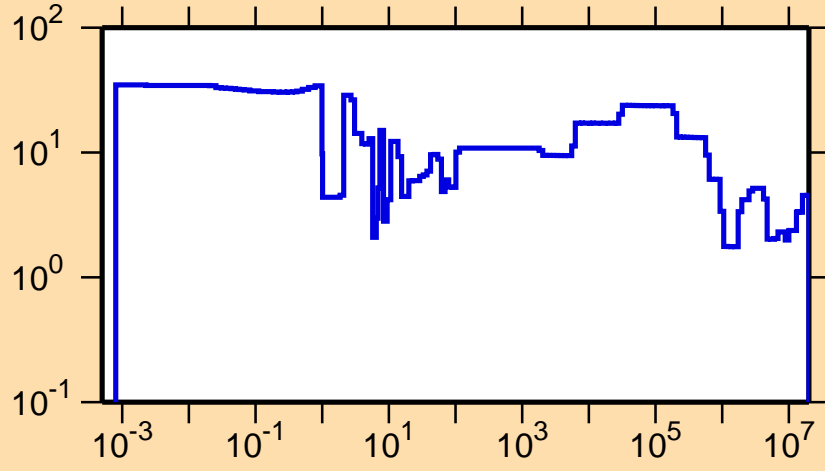
\Delta\sigma/\sigma vs. E for ^{108}\text{In}(n,\text{tot.})
