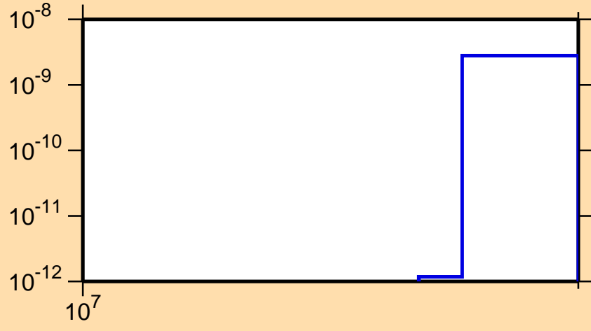
\sigma vs. E for ^{108}\text{In}(n,\text{pt})
