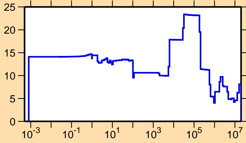
\Delta\sigma/\sigma vs. E for ^{108}\text{In}(n,\text{el.})
