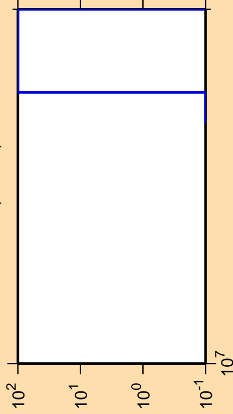
\Delta\sigma/\sigma vs. E for ^{108}\text{In}(\text{mt } 34)
