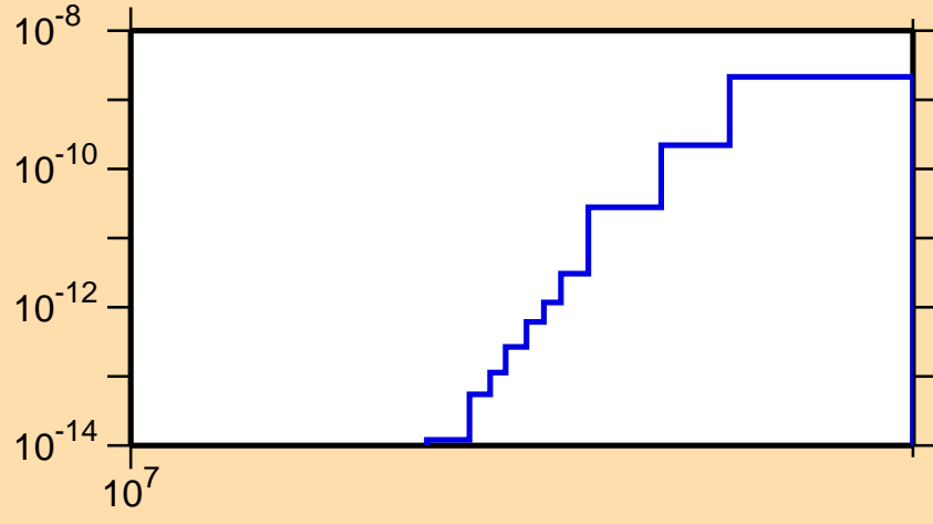
\sigma vs. E for ^{108}\text{In}(\text{mt117})
