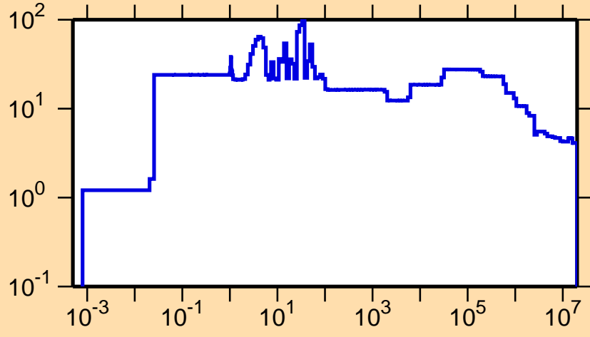
\Delta\sigma/\sigma vs. E for ^{108}\text{In}(n,\text{nonel.})
