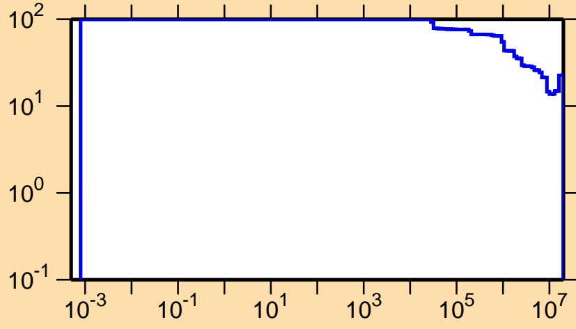
\Delta\sigma/\sigma vs. E for ^{108}\text{In}(n,p)
