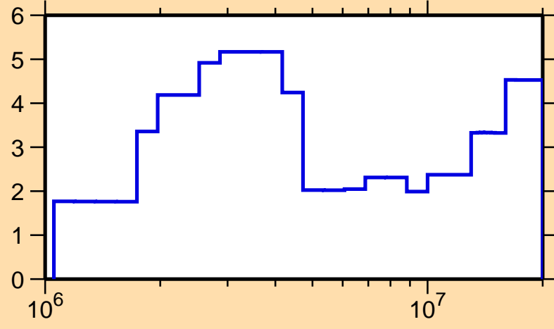
\Delta\sigma/\sigma vs. E for ^{108}\text{In}(n,\text{tot.})
