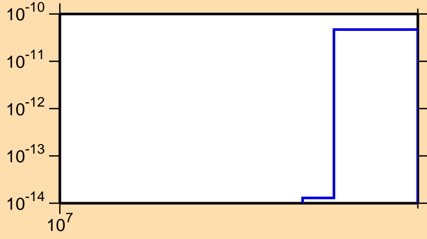
\sigma vs. E for ^{108}\text{In}(\text{mt } 34)
