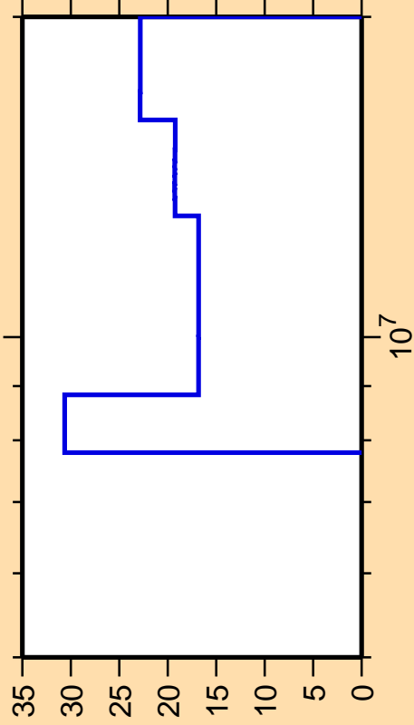
\Delta\sigma/\sigma vs. E for ^{108}\text{In}(n,2n)
