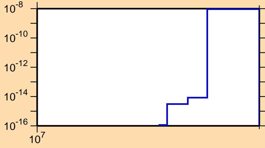
\sigma vs. E for ^{108}\text{In}(n,nt)
