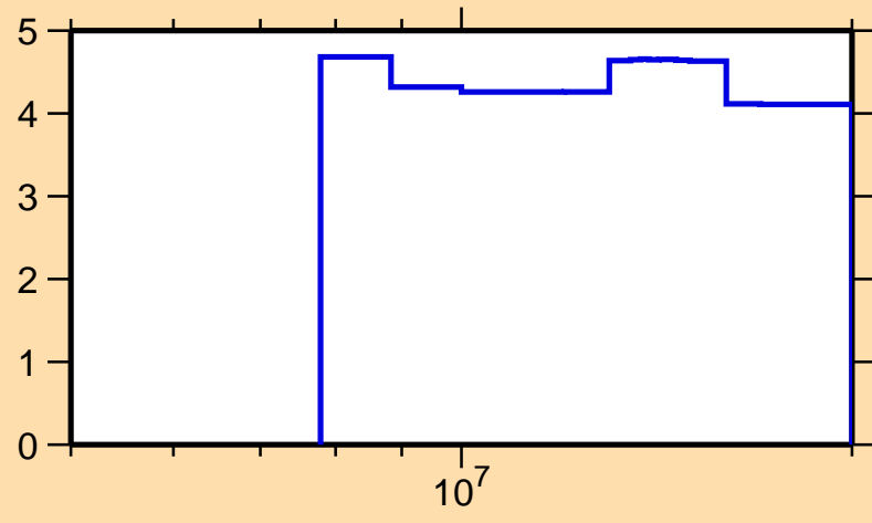
\Delta\sigma/\sigma vs. E for ^{108}\text{In}(n,\text{nonel.})
