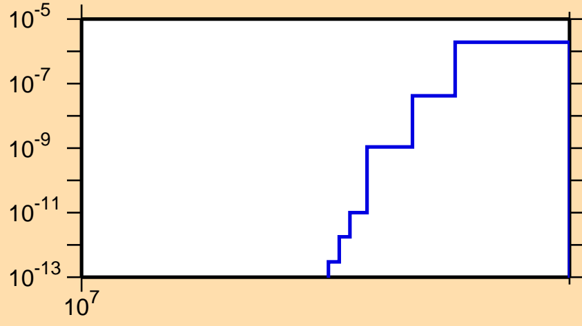
\sigma vs. E for ^{108}\text{In}(n,2n\alpha)
