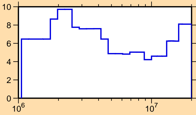
\Delta\sigma/\sigma vs. E for ^{108}\text{In}(n, el.)
