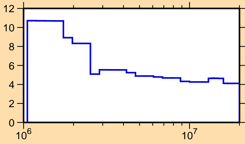
\Delta\sigma/\sigma vs. E for ^{108}\text{In}(n, \text{nonel.})
