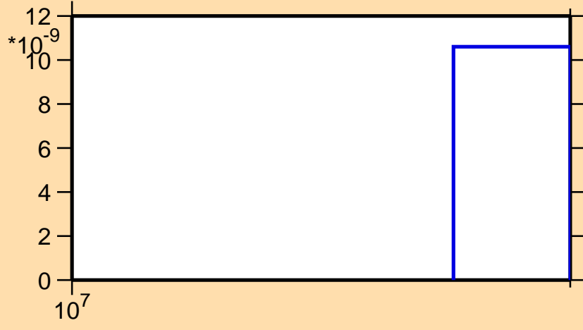
\sigma vs. E for ^{108}\text{In}(n,3n)
