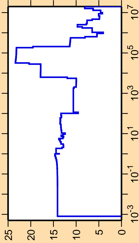
\Delta\sigma/\sigma vs. E for ^{108}\text{In}(n,\text{el.})
