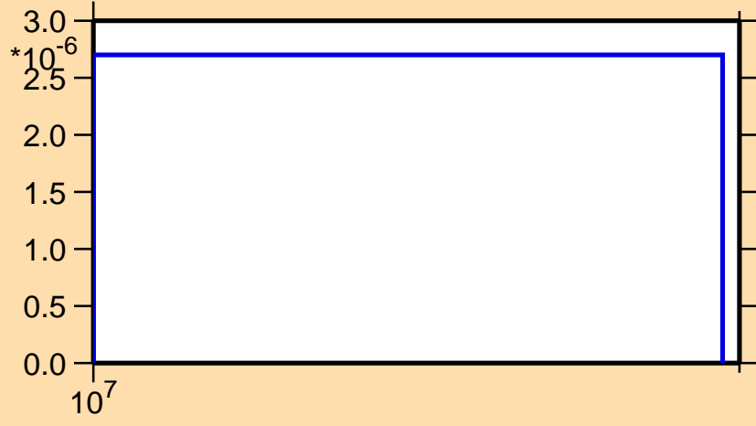
\sigma vs. E for ^{108}\text{In}(n,nd)
