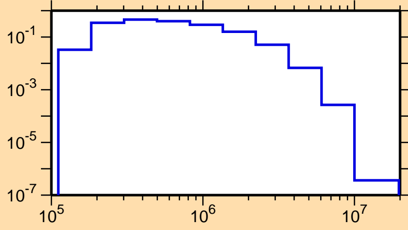
\sigma vs. E for ^{108}\text{In}(n,n_3)
