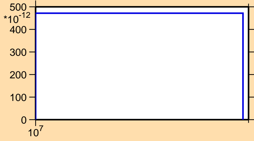
\sigma vs. E for ^{108}\text{In}(n,\text{pd})
