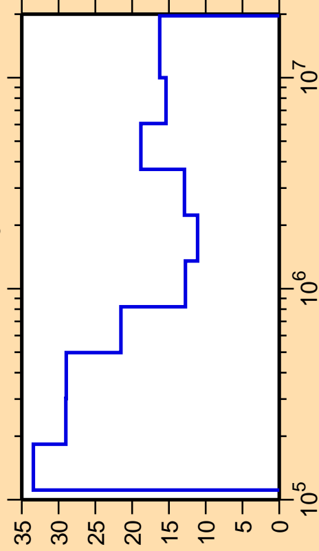
\Delta\sigma/\sigma vs. E for ^{108}\text{In}(n,n_3)
