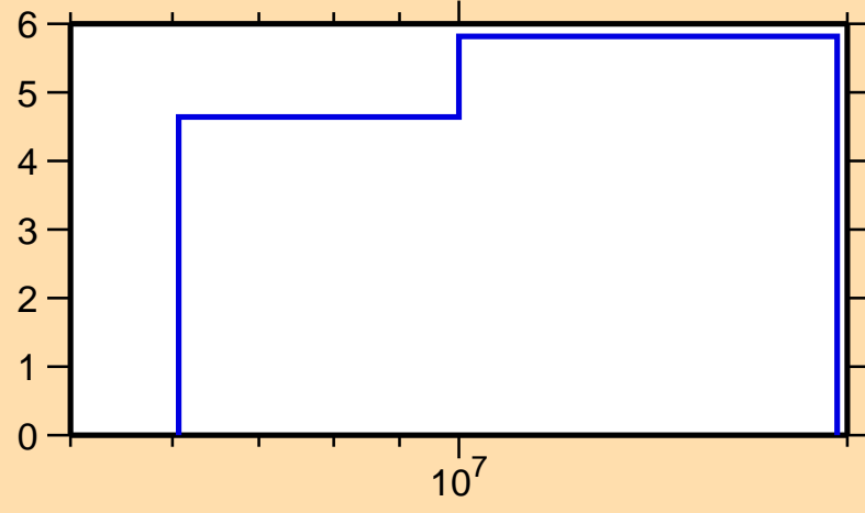
\Delta\sigma/\sigma vs. E for ^{108}\text{In}(n,\text{el.})
