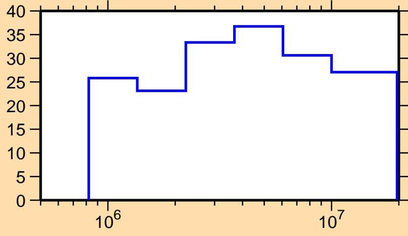
\Delta\sigma/\sigma vs. E for ^{108}\text{In}(n, n_1)
