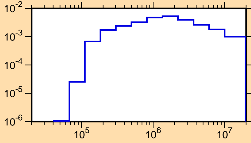
\sigma vs. E for ^{108}\text{In}(n,n_1)
