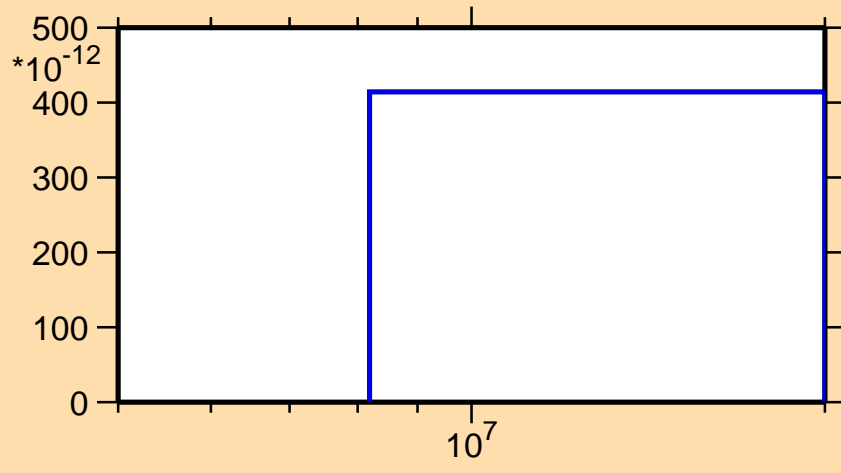
\sigma vs. E for ^{108}\text{In}(n,\text{pd})
