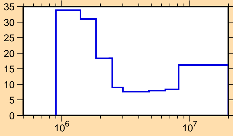
\Delta\sigma/\sigma vs. E for ^{108}\text{In}(n,n\text{cont.})
