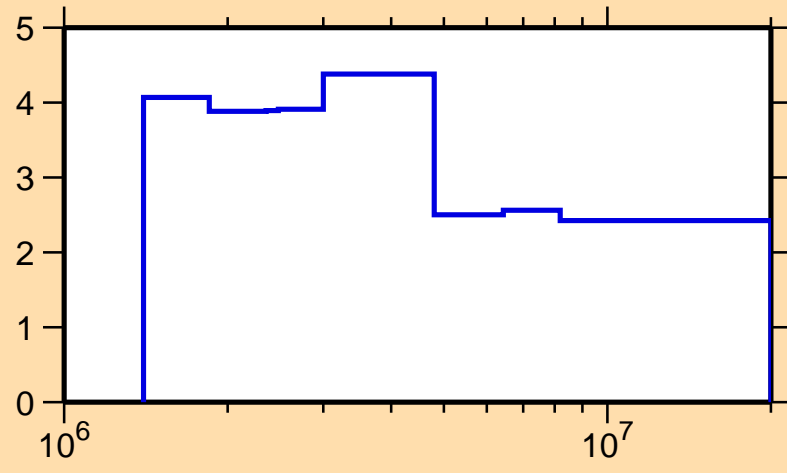
\Delta\sigma/\sigma vs. E for ^{109}\text{In}(n, n_{\text{nonel}})
