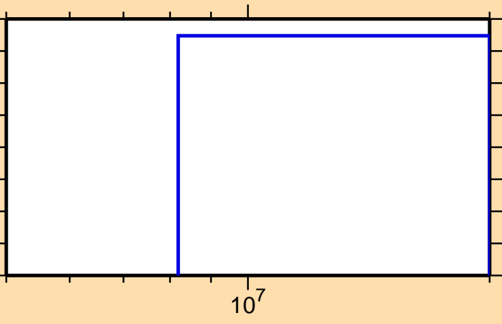
\sigma vs. E for ^{109}\text{In}(n,2np)
