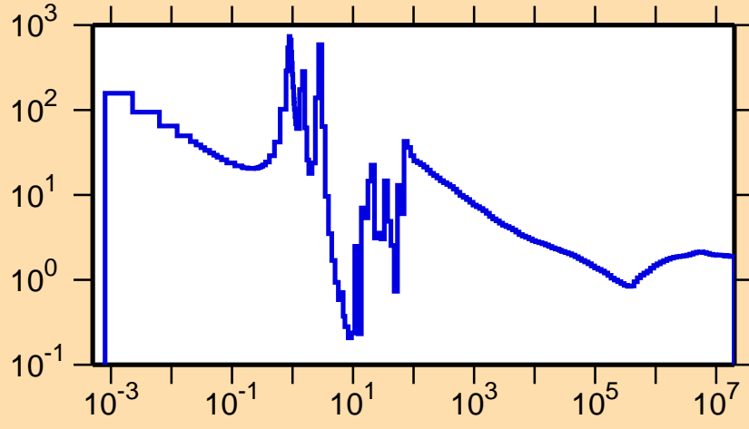
\sigma vs. E for ^{110}\text{In}(n,\text{nonel.})
