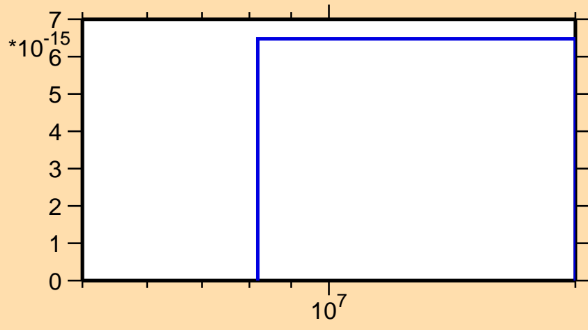
\sigma vs. E for ^{110}\text{In}(\text{mt } 34)
