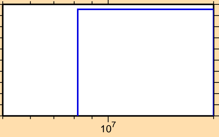
\sigma vs. E for ^{110}\text{In}(n,nt)
