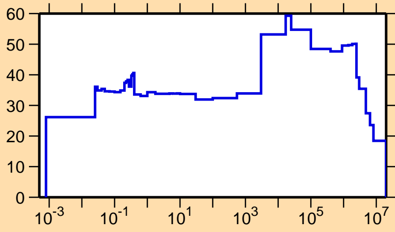
\Delta\sigma/\sigma vs. E for ^{110}\text{In}(n,p)
