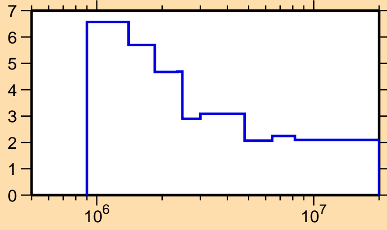
\Delta\sigma/\sigma vs. E for ^{110}\text{In}(n, n_{\text{nonel}})
