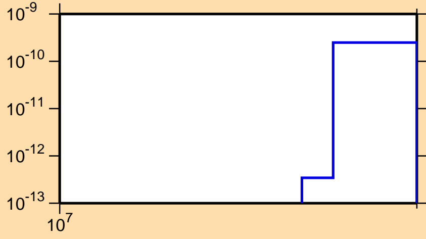
\sigma vs. E for ^{110}\text{In}(n,\text{pd})
