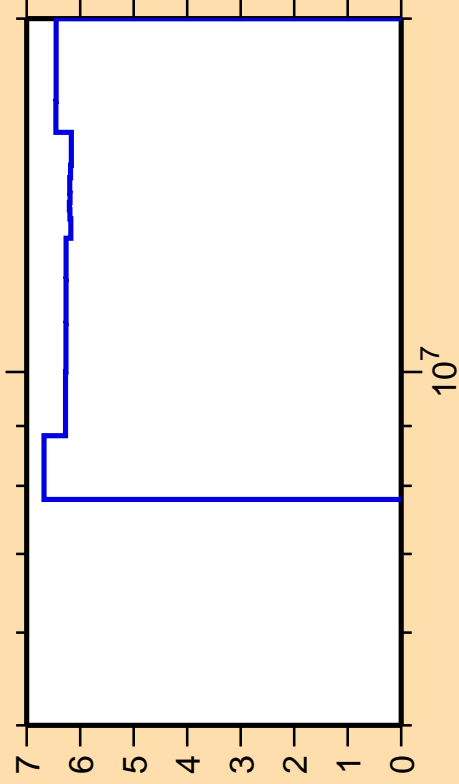
\Delta\sigma/\sigma vs. E for ^{110}\text{In}(n,2n)
