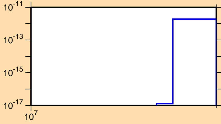
\sigma vs. E for ^{110}\text{In} (mt 34)
