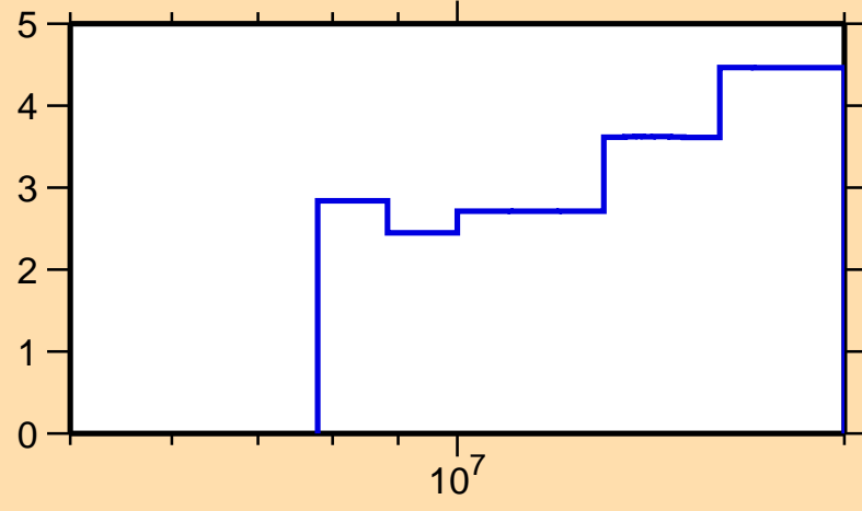
\Delta\sigma/\sigma vs. E for ^{110}\text{In}(n,\text{el.})
