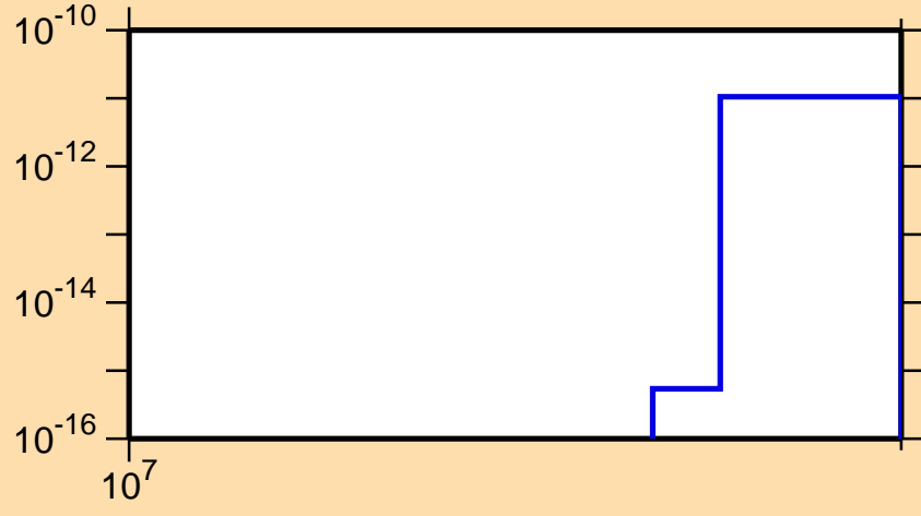
\sigma vs. E for ^{110}\text{In}(n,\text{pt})
