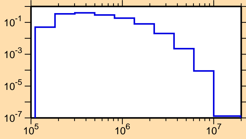
\sigma vs. E for ^{110}\text{In}(n,n_2)
