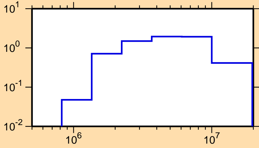
\sigma vs. E for ^{110}\text{In}(n,n\text{cont.})
