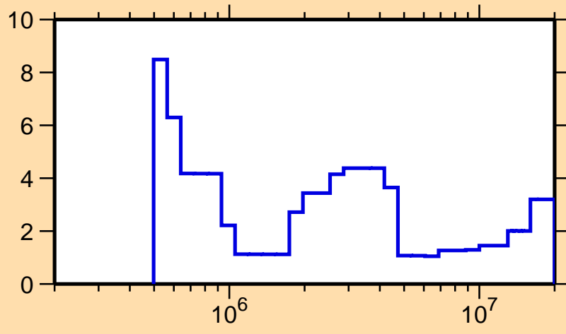
\Delta\sigma/\sigma vs. E for ^{111}\text{In}(n,\text{tot.})
