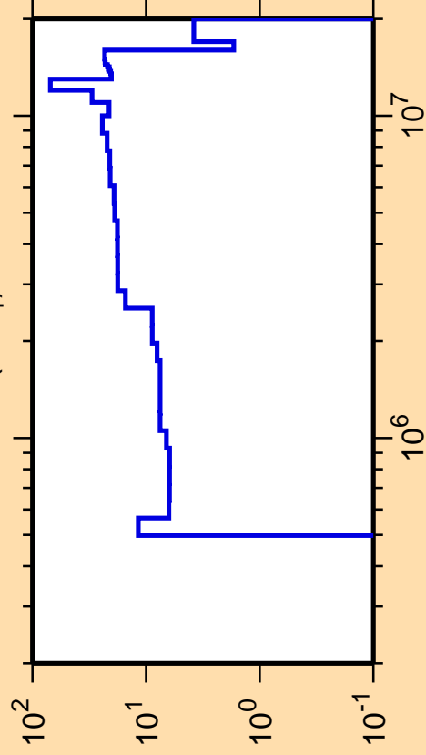
\Delta\sigma/\sigma vs. E for ^{111}\text{In}(n,n_1)
