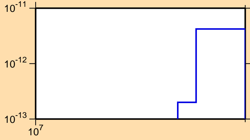
\sigma vs. E for ^{111}\text{In}(\text{mt117})
