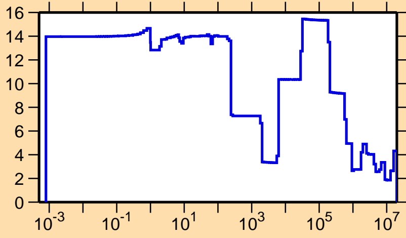
\Delta\sigma/\sigma vs. E for ^{111}\text{In}(n,\text{el.})
