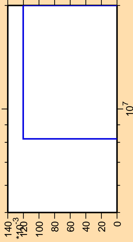
\Delta\sigma/\sigma vs. E for ^{111}\text{In} (mt 45)
