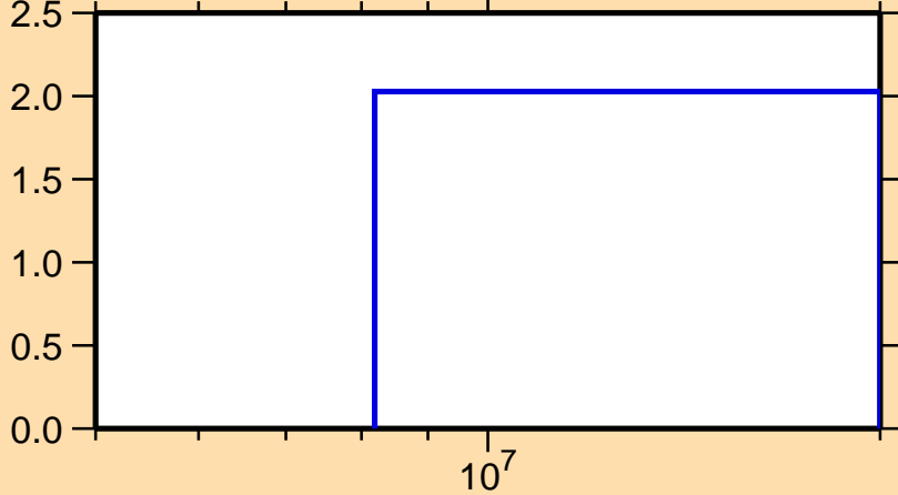
\Delta\sigma/\sigma vs. E for ^{111}\text{In}(n,\text{el.})
