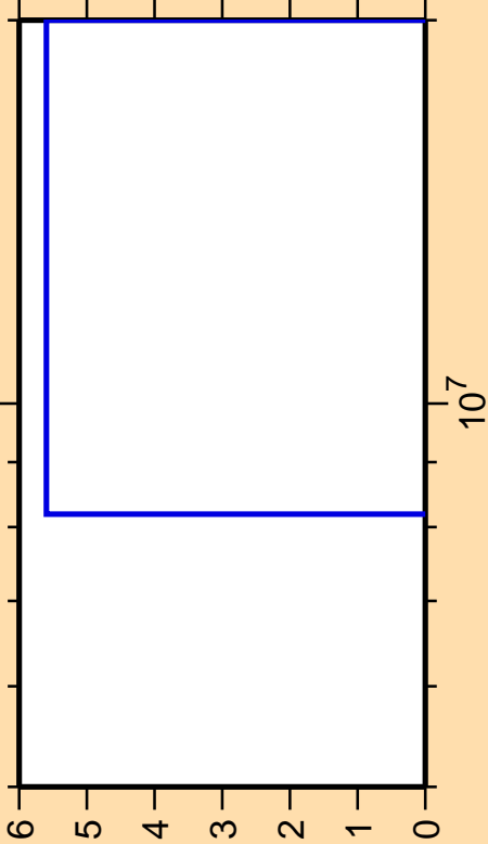
\Delta\sigma/\sigma vs. E for ^{111}\text{In}(n,2n)
