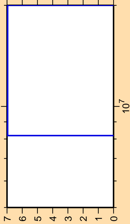
\Delta\sigma/\sigma vs. E for ^{111}\text{In}(n,2n\alpha)
