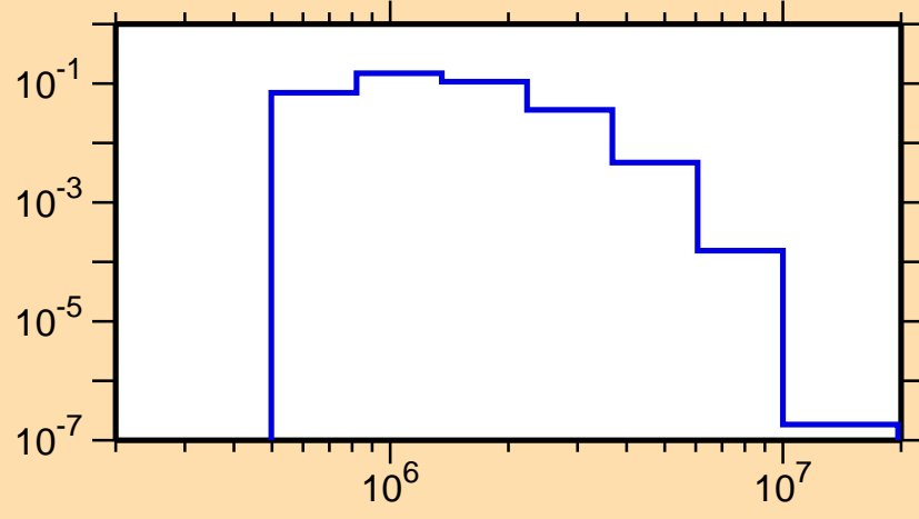
\sigma vs. E for ^{111}\text{In}(n,n_3)
