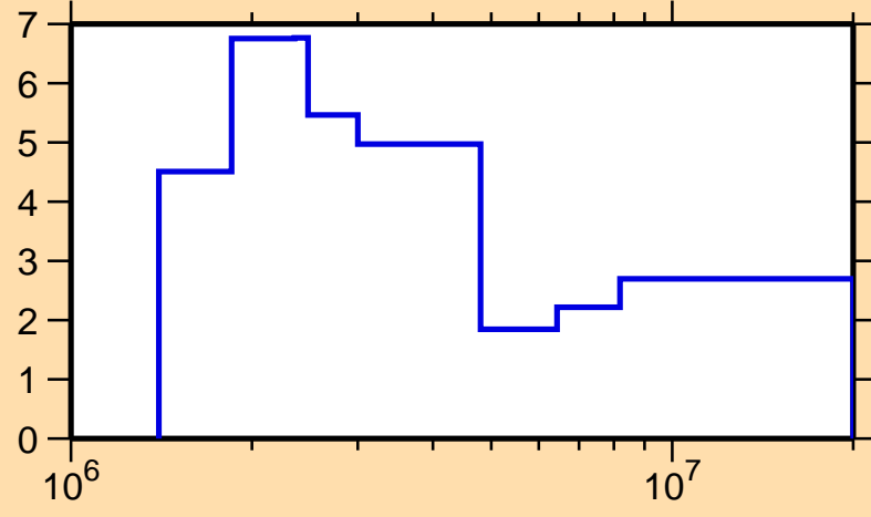
\Delta\sigma/\sigma vs. E for ^{111}\text{In}(n, el.)
