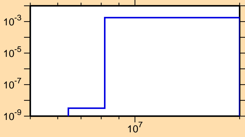
\sigma vs. E for ^{111}\text{In}(n,n\alpha)
