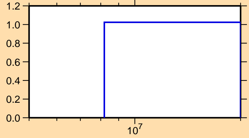
\sigma vs. E for ^{111}\text{In}(n,2n)
