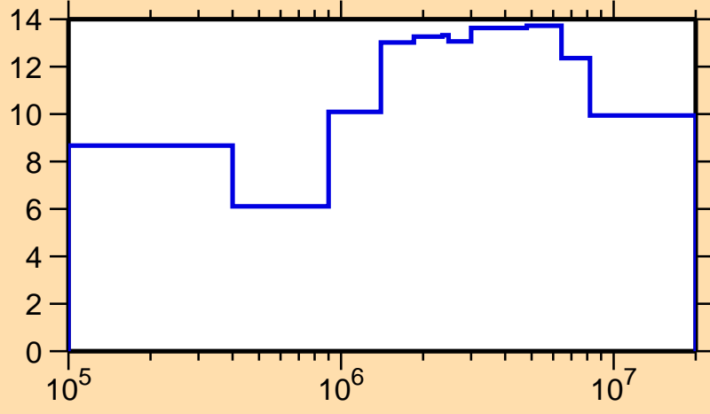
\Delta\sigma/\sigma vs. E for ^{112}\text{In}(n,n_1)
