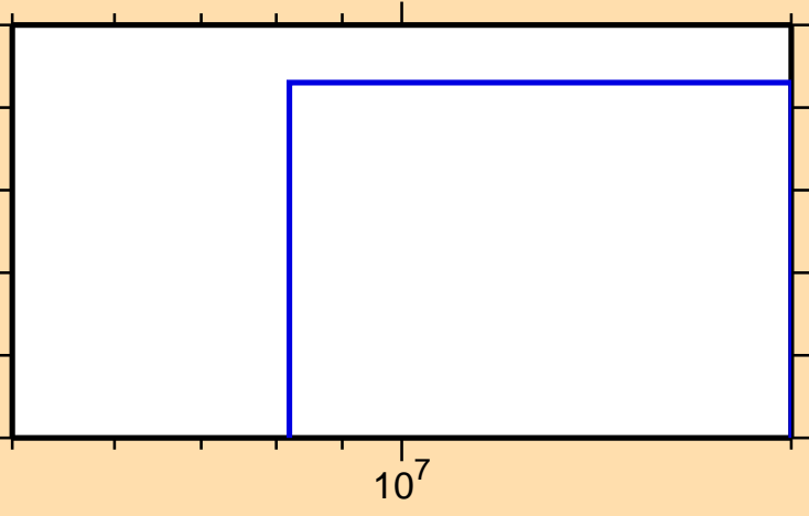
\sigma vs. E for ^{112}\text{In}(n,\text{He3})
