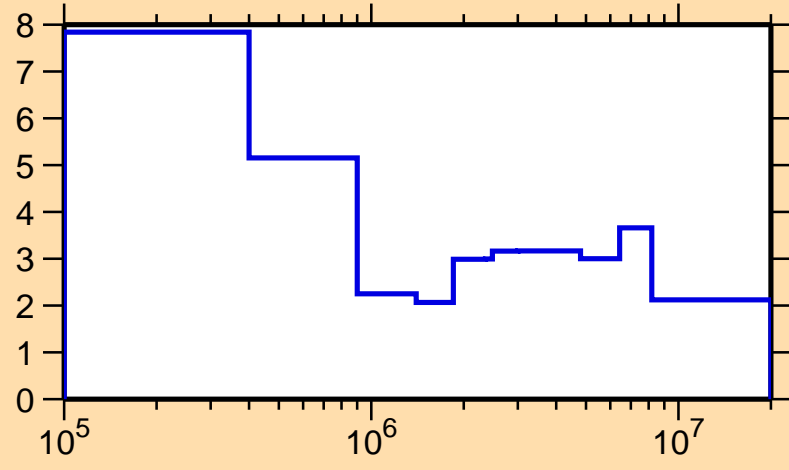
\Delta\sigma/\sigma vs. E for ^{112}\text{In}(n,\text{el.})
