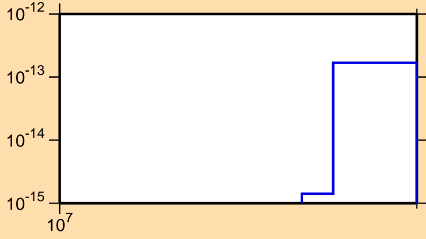
\sigma vs. E for ^{112}\text{In}(\text{mt117})
