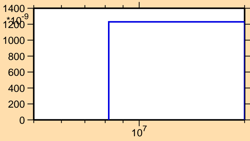
\sigma vs. E for ^{112}\text{In}(n,\text{nd})
