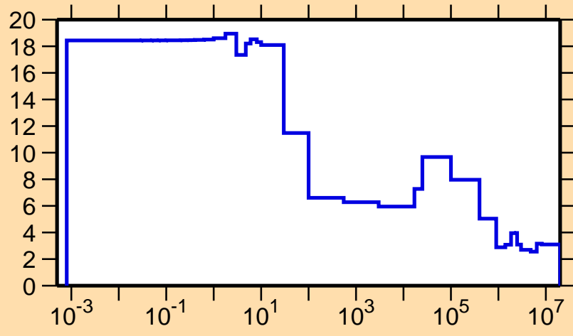
\Delta\sigma/\sigma vs. E for ^{112}\text{In}(n,el.)
