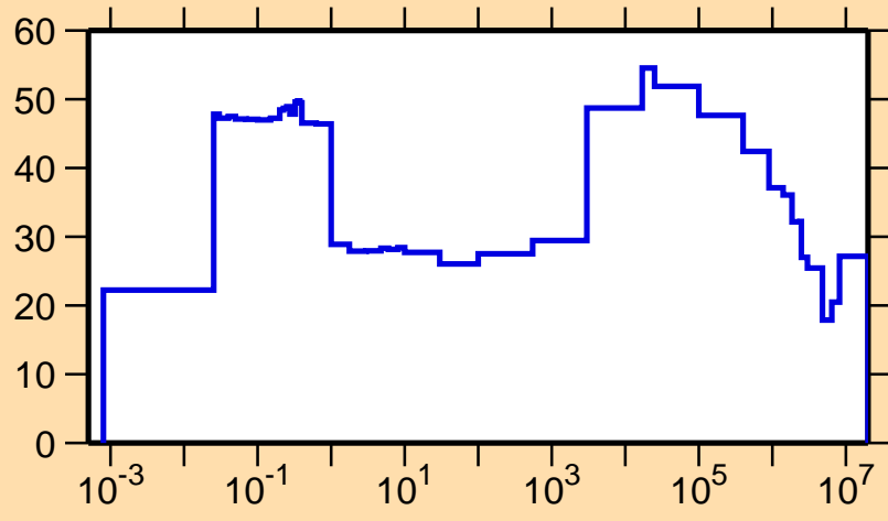
\Delta\sigma/\sigma vs. E for ^{112}\text{In}(n,p)
