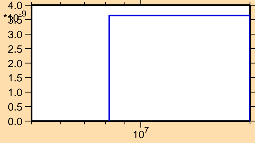
\sigma vs. E for ^{112}\text{In}(n,\text{He3})
