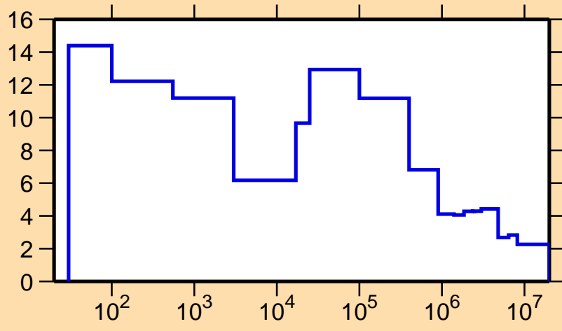
\Delta\sigma/\sigma vs. E for ^{112}\text{In}(n,\text{nonel.})
