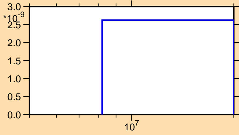
\sigma vs. E for ^{112}\text{In}(n,2n\alpha)
