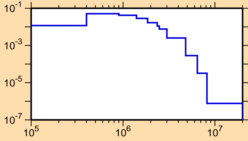
\sigma vs. E for ^{112}\text{In}(n,n_4)
