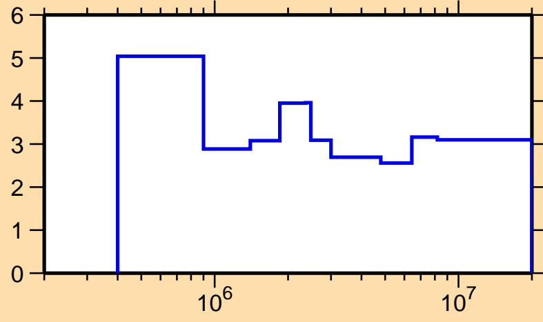
\Delta\sigma/\sigma vs. E for ^{112}\text{In}(n, el.)
