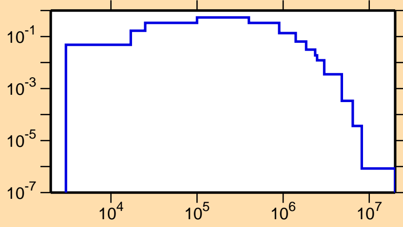
\sigma vs. E for ^{112}\text{In}(n,n_2)
