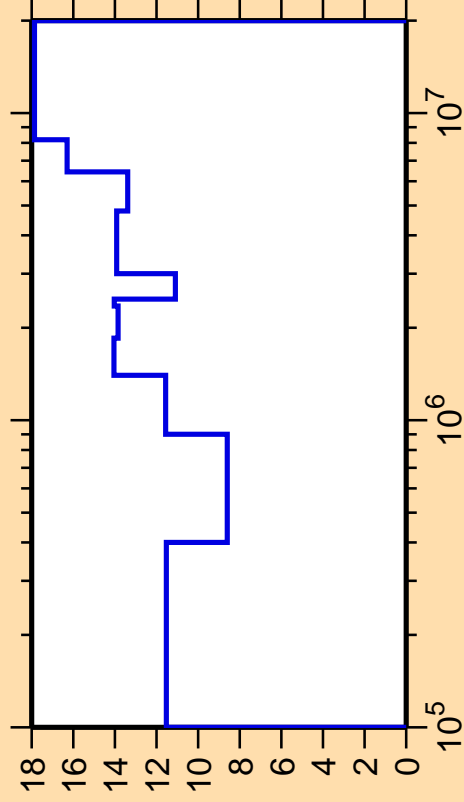
\Delta\sigma/\sigma vs. E for ^{112}\text{In}(n,n_4)
