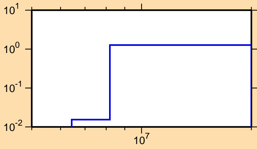
\sigma vs. E for ^{112}\text{In}(n,2n)
