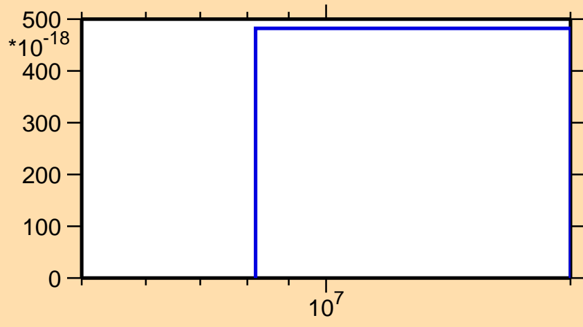
\sigma vs. E for ^{112}\text{In}(n,\text{pd})
