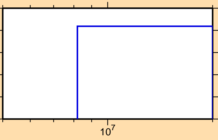
\sigma vs. E for ^{112}\text{In}(n,2np)
