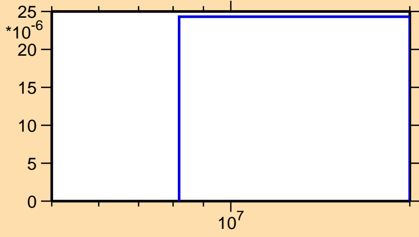
\sigma vs. E for ^{112}\text{In}(n,3n)
