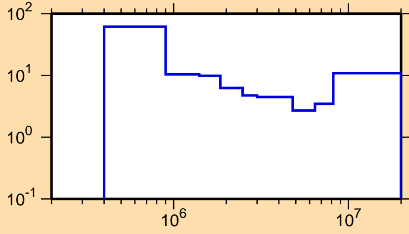
\Delta\sigma/\sigma vs. E for ^{112}\text{In}(n,n\text{cont.})
