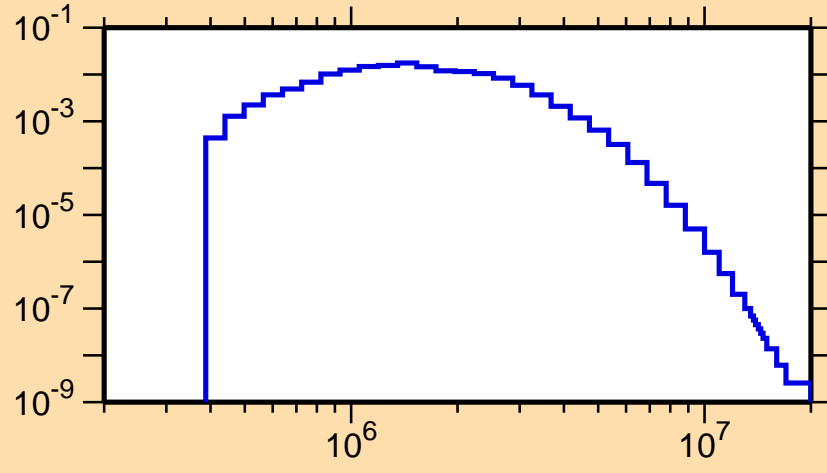
\sigma vs. E for ^{113}\text{In}(n,n_1)
