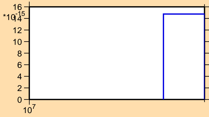
\sigma vs. E for ^{113}\text{In}(\text{mt } 45)
