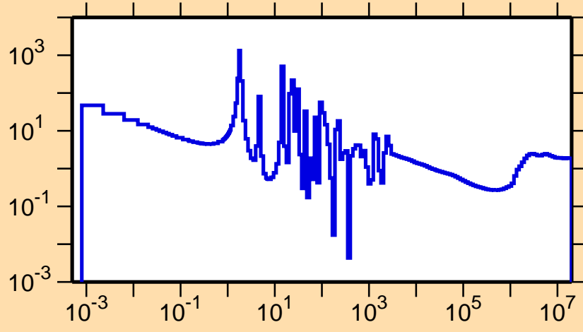
\sigma vs. E for ^{113}\text{In}(n,\text{nonel.})
