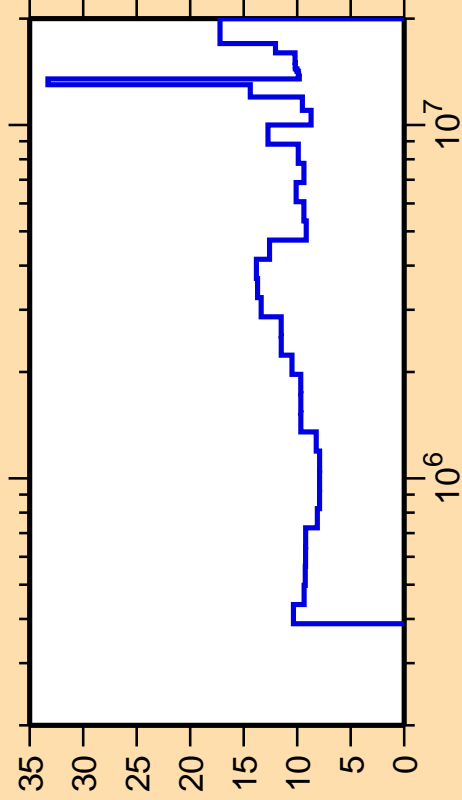
\Delta\sigma/\sigma vs. E for ^{113}\text{In}(n,n_1)
