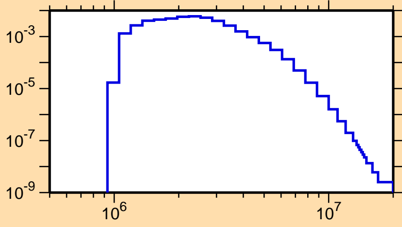
\sigma vs. E for ^{113}\text{In}(n,n_4)
