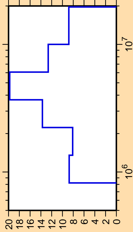
\Delta\sigma/\sigma vs. E for ^{113}\text{In}(n,n_4)
