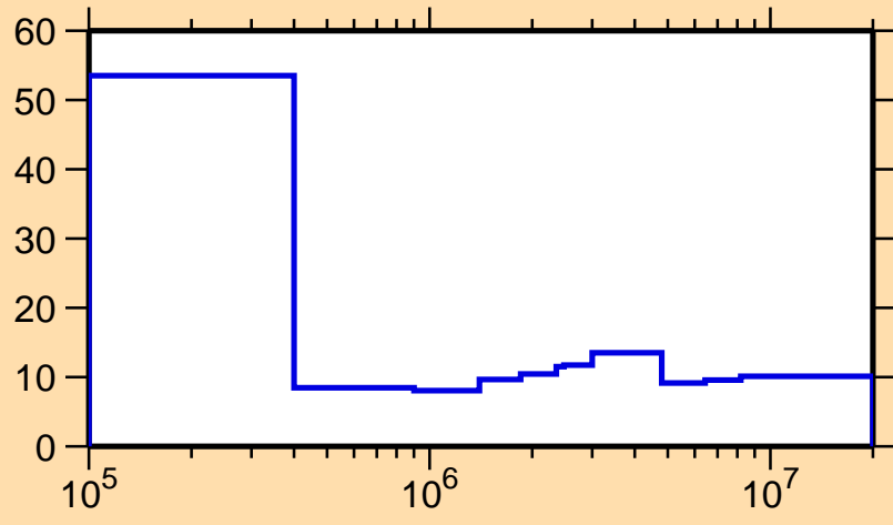
\Delta\sigma/\sigma vs. E for ^{113}\text{In}(n,n_1)
