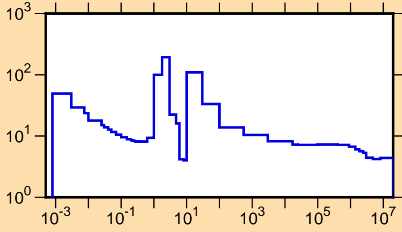
\sigma vs. E for ^{113}\text{In}(n,\text{tot.})
