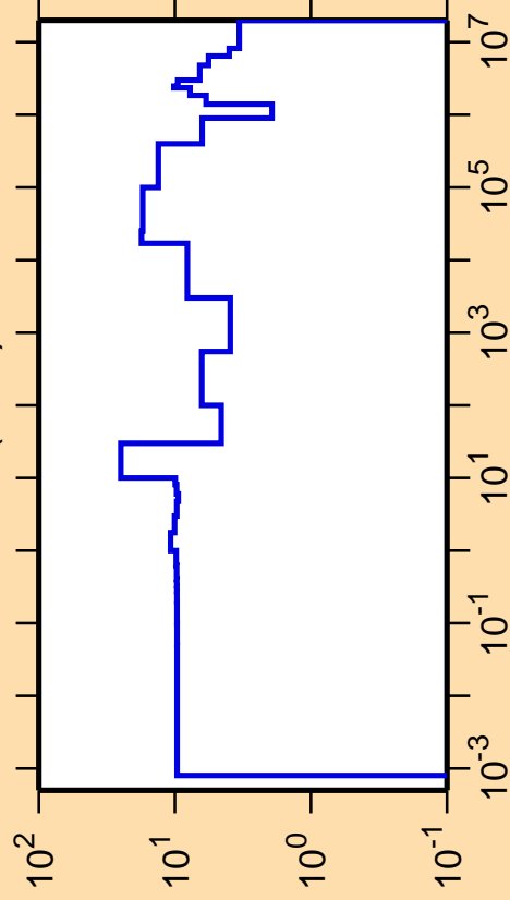
\Delta\sigma/\sigma vs. E for ^{113}\text{In}(n,\text{el.})
