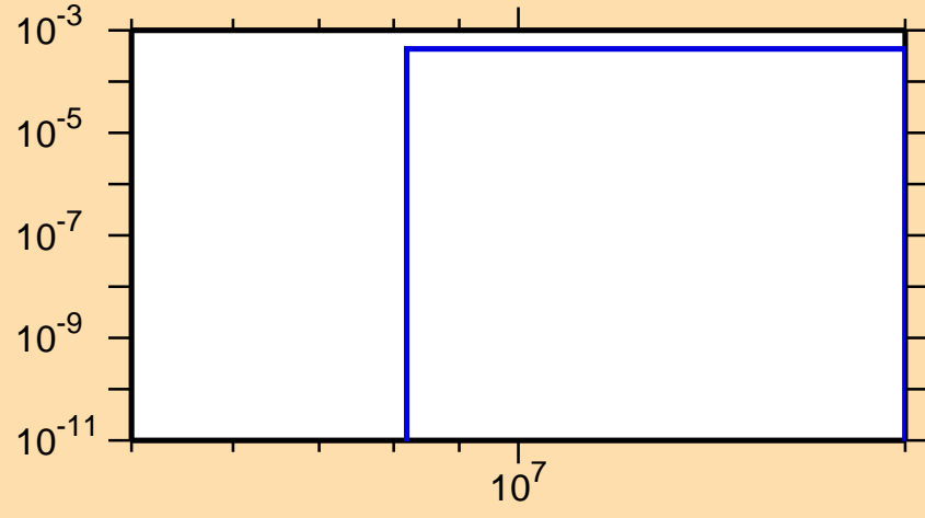
\sigma vs. E for ^{113}\text{In}(n,n\alpha)
