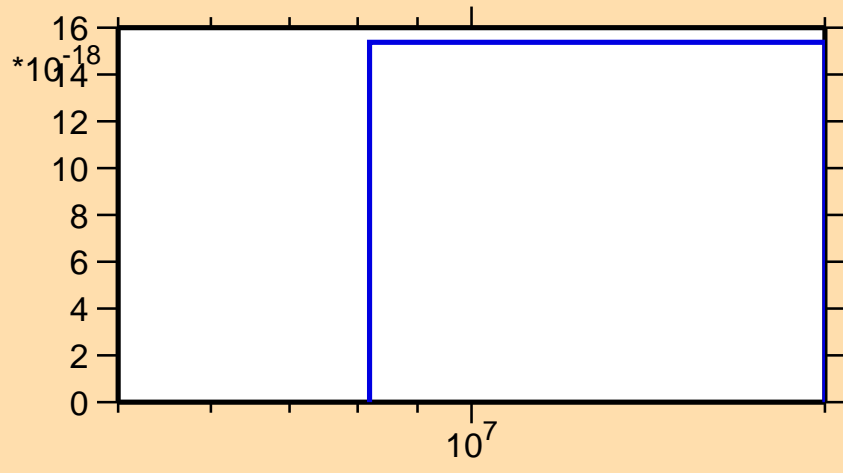
\sigma vs. E for ^{113}\text{In}(n,\text{pd})
