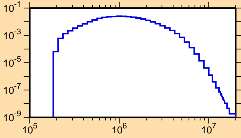
\sigma vs. E for ^{114}\text{In}(n,n_1)
