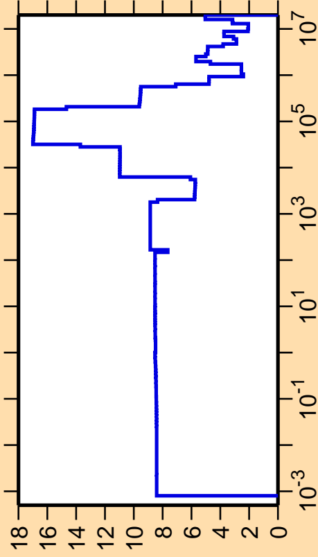
\Delta\sigma/\sigma vs. E for ^{114}\text{In}(n,\text{el.})
