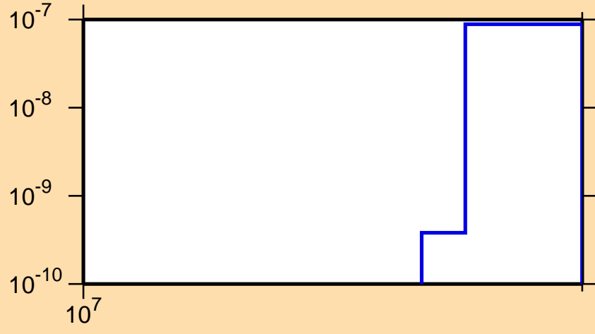
\sigma vs. E for ^{114}\text{In}(n,2n\alpha)
