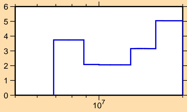
\Delta\sigma/\sigma vs. E for ^{114}\text{In}(n,\text{el.})
