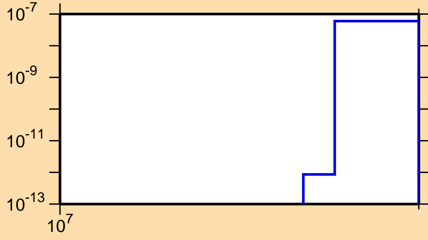
\sigma vs. E for ^{114}\text{In}(n,nt)
