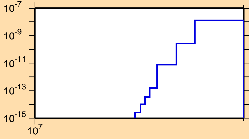
\sigma vs. E for ^{114}\text{In}(n,\text{He3})
