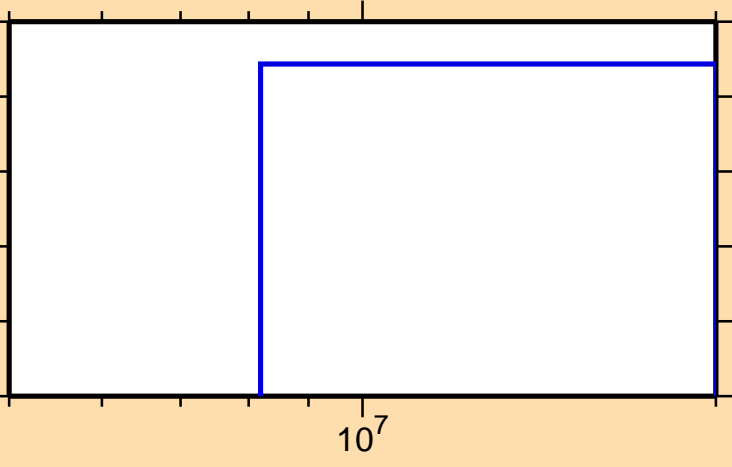
\sigma vs. E for ^{114}\text{In}(n,2np)
