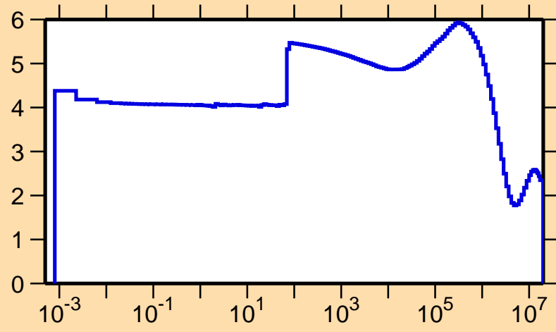
\sigma vs. E for ^{114}\text{In}(n,\text{el.})
