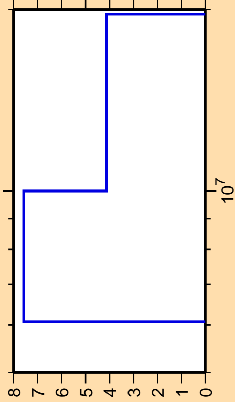
\Delta\sigma/\sigma vs. E for ^{114}\text{In}(n,2n)
