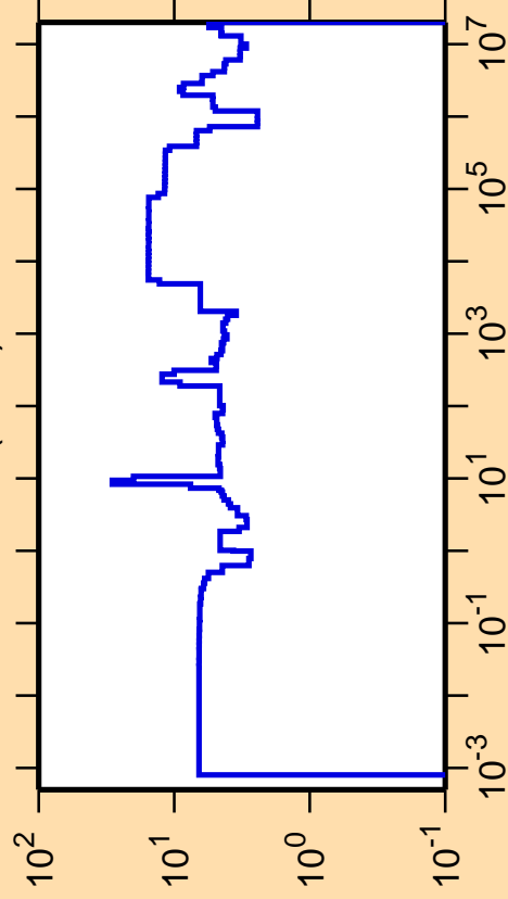
\Delta\sigma/\sigma vs. E for ^{115}\text{In}(n,\text{el.})
