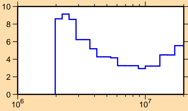
\Delta\sigma/\sigma vs. E for ^{115}\text{In}(n,el.)
