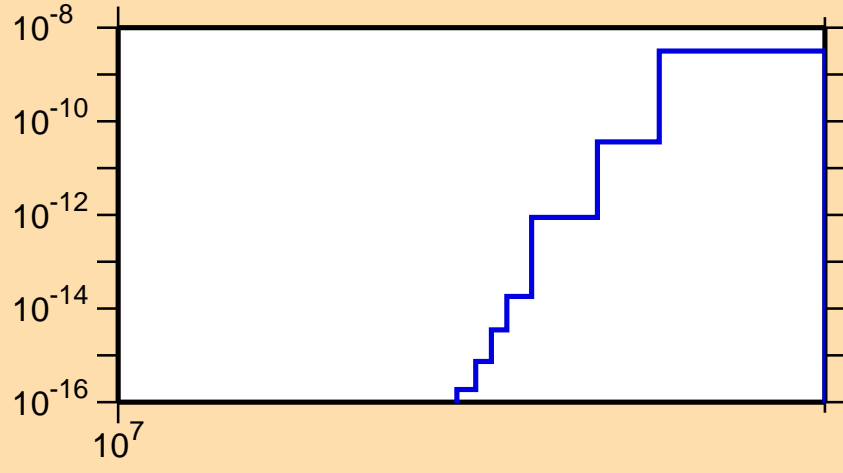
\sigma vs. E for ^{115}\text{In}(n,\text{He3})
