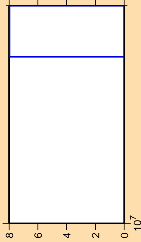
\Delta\sigma/\sigma vs. E for ^{115}\text{In}(n,p\alpha)
