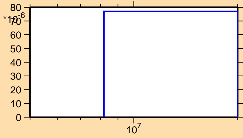
\sigma vs. E for ^{115}\text{In}(n,t)
