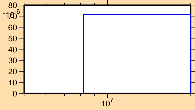
\sigma vs. E for ^{115}\text{In}(n,n\alpha)
