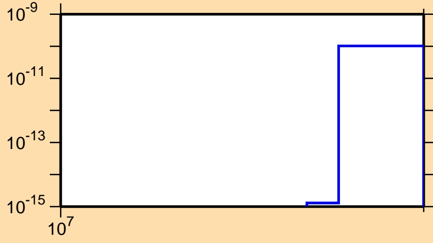
\sigma vs. E for ^{115}\text{In}(n,2n\alpha)
