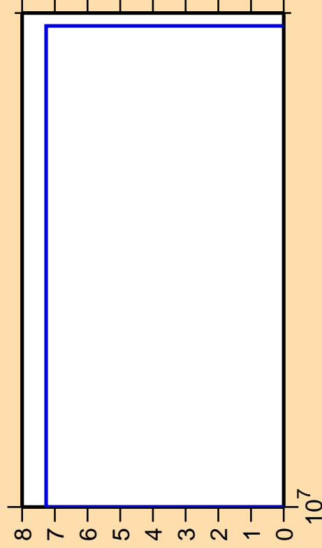
\Delta\sigma/\sigma vs. E for ^{115}\text{In}(n,\text{He}3)
