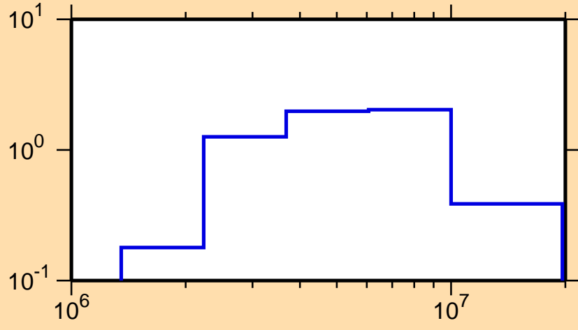
\sigma vs. E for ^{115}\text{In}(n,n\text{cont.})
