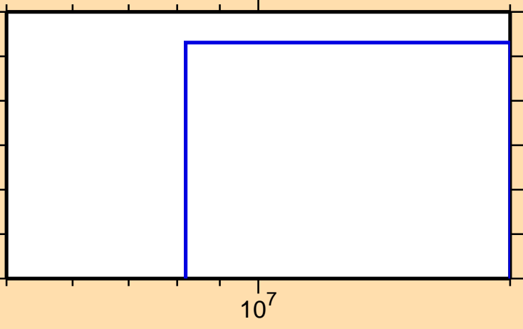
\sigma vs. E for ^{115}\text{In}(n,3n)
