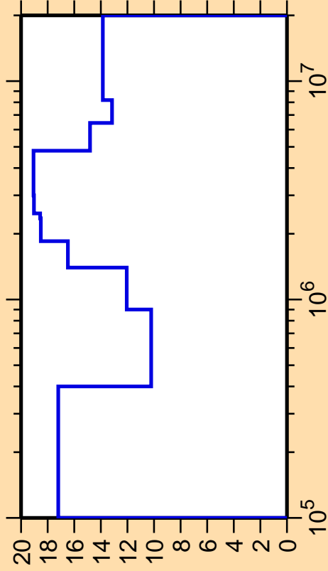
\Delta\sigma/\sigma vs. E for ^{116}\text{In}(n,n_2)
