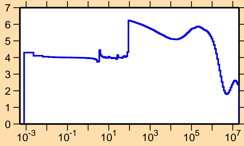
\sigma vs. E for ^{116}\text{In}(n,\text{el.})
