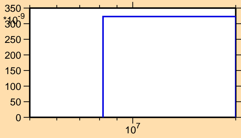
\sigma vs. E for ^{116}\text{In}(n,nd)
