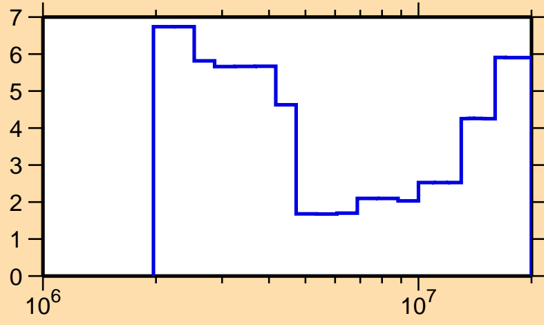
\Delta\sigma/\sigma vs. E for ^{117}\text{In}(n, el.)
