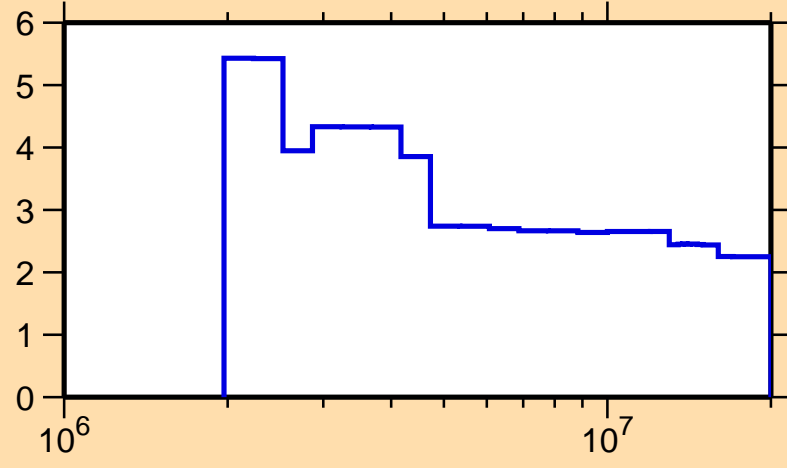
\Delta\sigma/\sigma vs. E for ^{117}\text{In}(n, n_{\text{nonel}})
