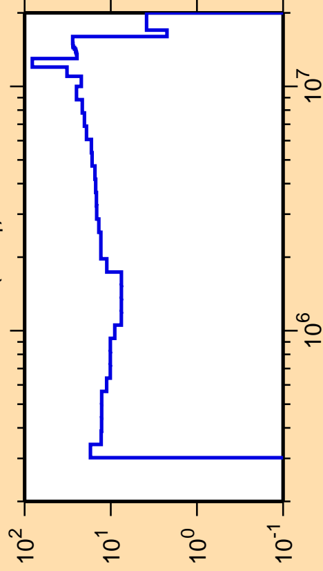
\Delta\sigma/\sigma vs. E for ^{117}\text{In}(n,n_1)
