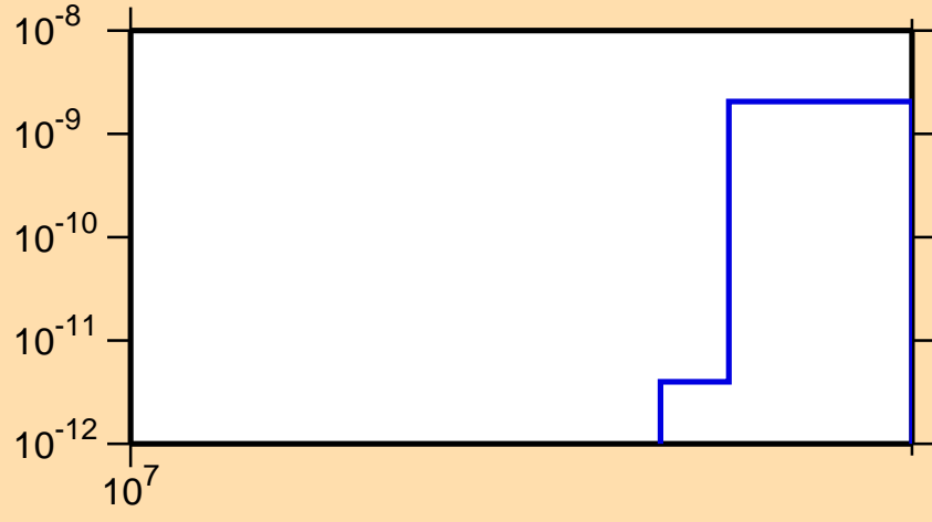
\sigma vs. E for ^{118}\text{In}(n,2n\alpha)
