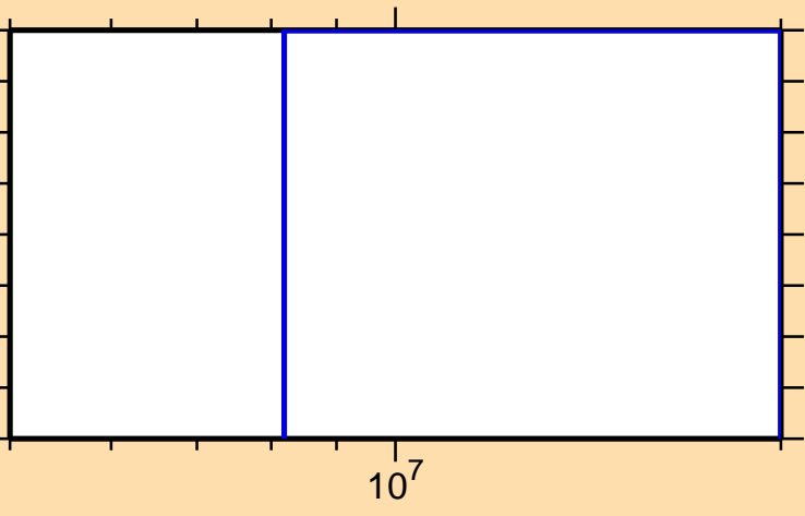
\sigma vs. E for ^{118}\text{In}(n,2np)
