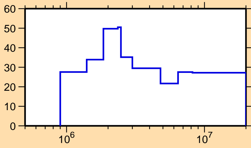
\Delta\sigma/\sigma vs. E for ^{118}\text{In}(n,n_1)
