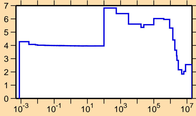
\sigma vs. E for ^{118}\text{In}(n,\text{el.})
