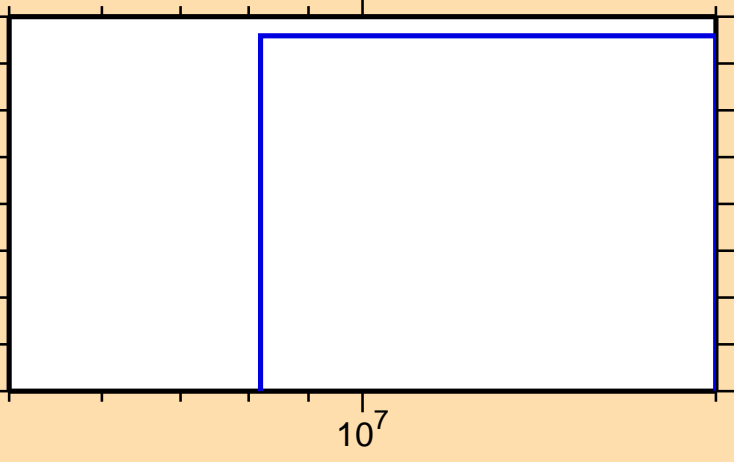
\sigma vs. E for ^{118}\text{In}(n,t)
