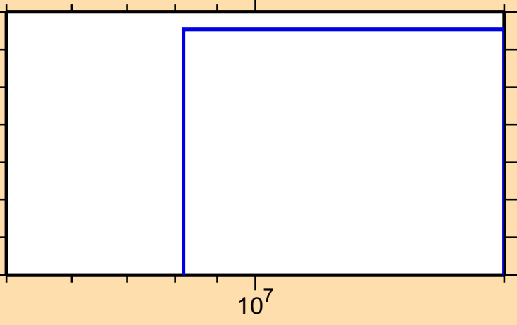
\sigma vs. E for ^{118}\text{In}(n,n\alpha)
