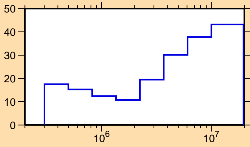
\Delta\sigma/\sigma vs. E for ^{119}\text{In}(n,n_1)
