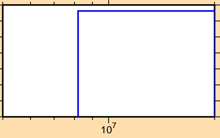
\sigma vs. E for ^{119}\text{In}(n,nt)
