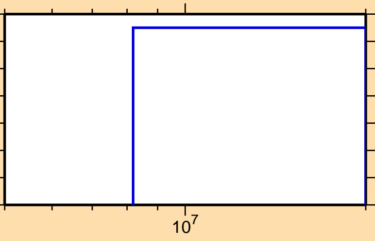
\sigma vs. E for ^{119}\text{In}(n,3n)
